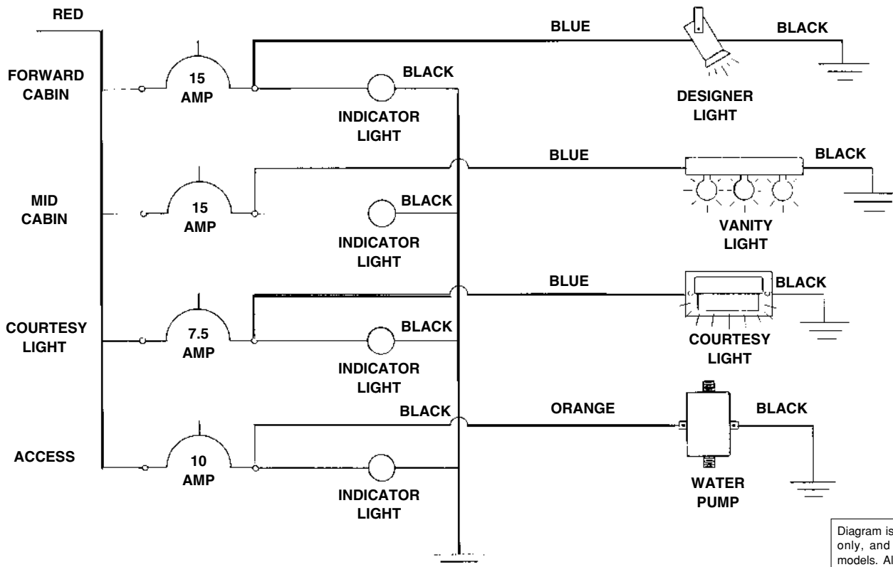
FIGURE 2.1 - TYPICAL 12-VOLT DC CABIN SCHEMATIC
