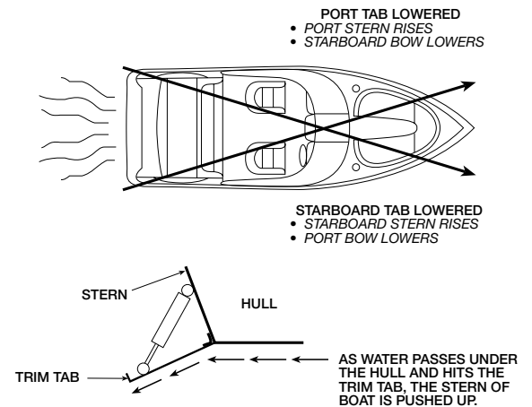
FIGURE 3.4 - TRIMMING WITH TRIM TABS
