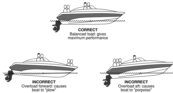
FIGURE 3.2 – LOADING PASSENGERS
