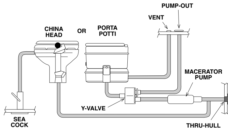
FIGURE 2.7 - CHINA HEAD OR MACERATOR HEAD TO OVERBOARD DISCHARGE
