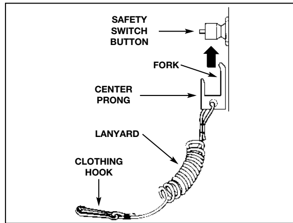
FIGURE 2.9 IGNITION INTERRUPTER WITH LANYARD
