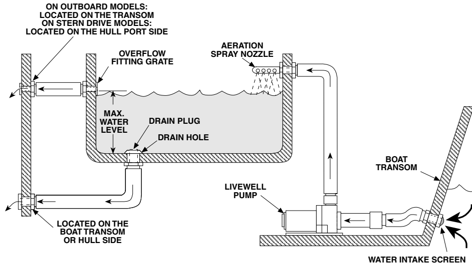
FIGURE 2.10 MANUAL LIVEWELL
