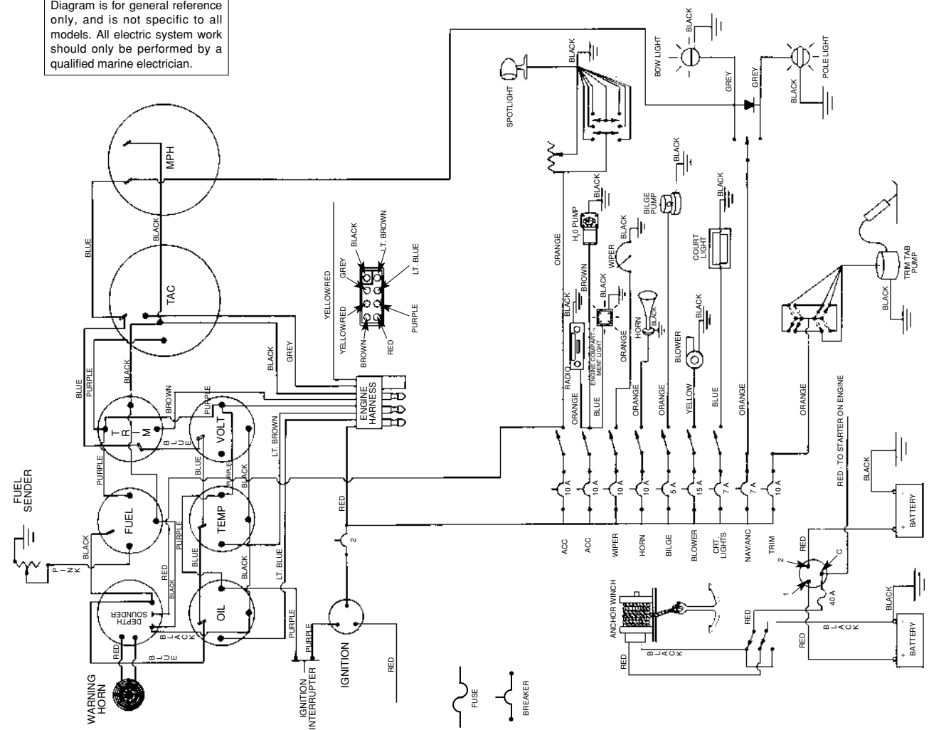
FIGURE 2.2 - TYPICAL SINGLE ENGINE SCHEMATIC
