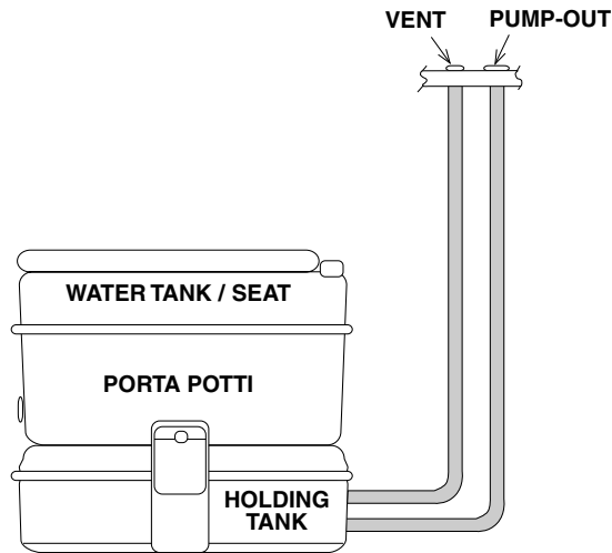
FIGURE 2.6 – ENCLOSED MARINE HEAD WITH PUMP-OUT
