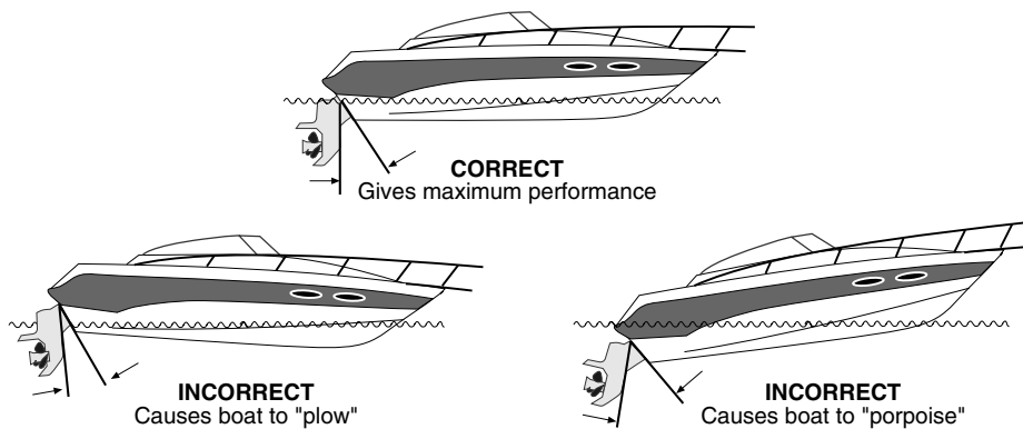
FIGURE 3.3 - TRIM / MOTOR ANGLE
