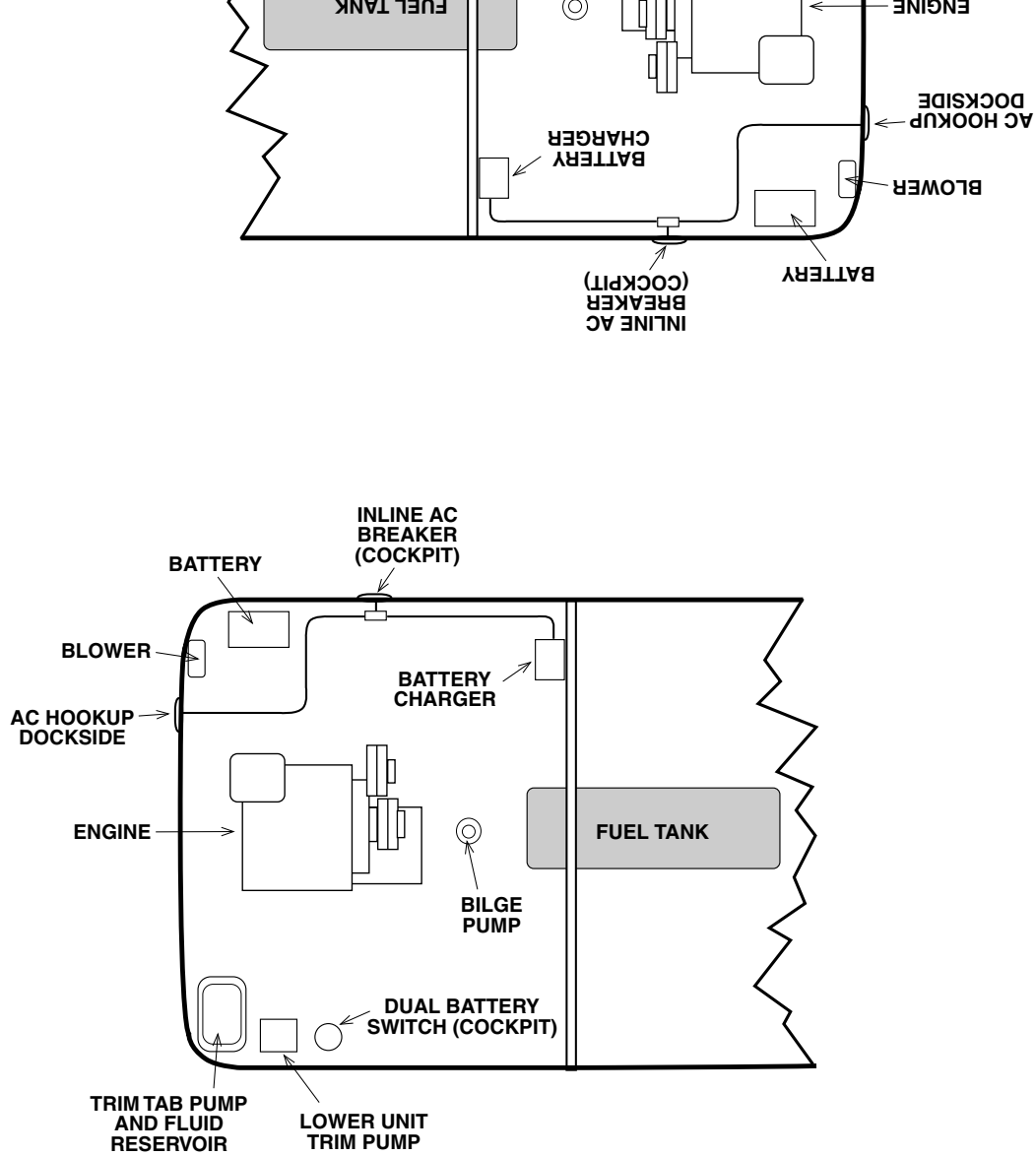
FIGURE 2.8 – TYPICAL SINGLE ENGINE COMPARTMENT
