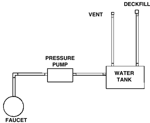
FIGURE 2.5 – TYPICAL PLUMBING DIAGRAM
