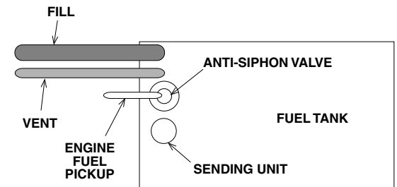
FIGURE 2.4 – FUEL SYSTEM
