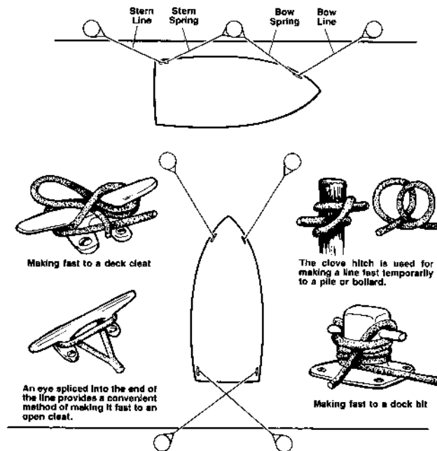
FIGURE 3.1 - MOORING LINES
